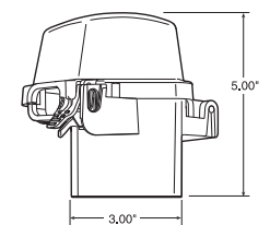
SINGLE GANG DEEP COVER
