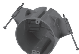
3-1/2" round new work non-metallic ceiling box 3-1/2" diameter x 2-3/4" (89mm x 70mm)
