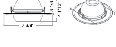
RT603WH White Eyeball Uses BR/PAR30 Lamps Order Code: 79551
