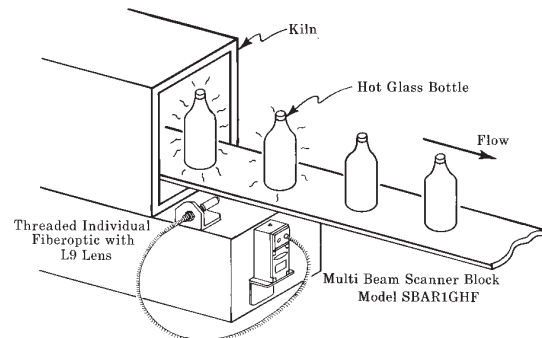
Counting bottles during the manufacturing process by detecting infrared (heat) radiation with an ambient light receiver.
