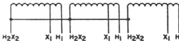
3-Phase Wiring Diagram
