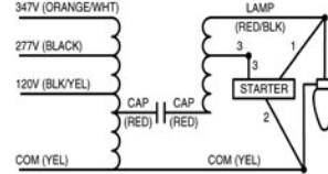
Wiring Diagram 3
