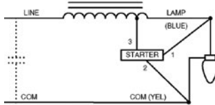
Wiring Diagram 7
