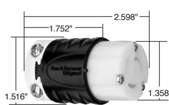
15A Connector
