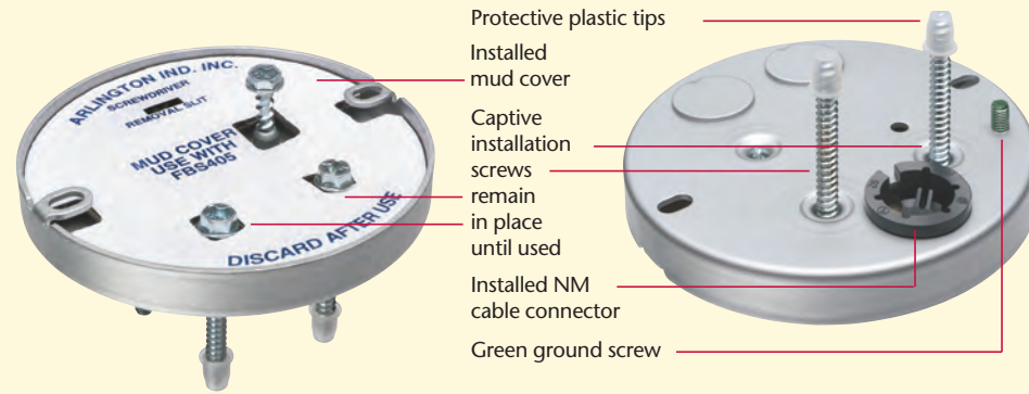
FBS405T inside view
