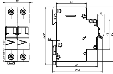
1+N-pole, 2-pole
