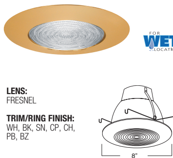
AF642CL-WH (SOCKET SUPPORTING) REFLECTOR W/ FRESNEL LENS
