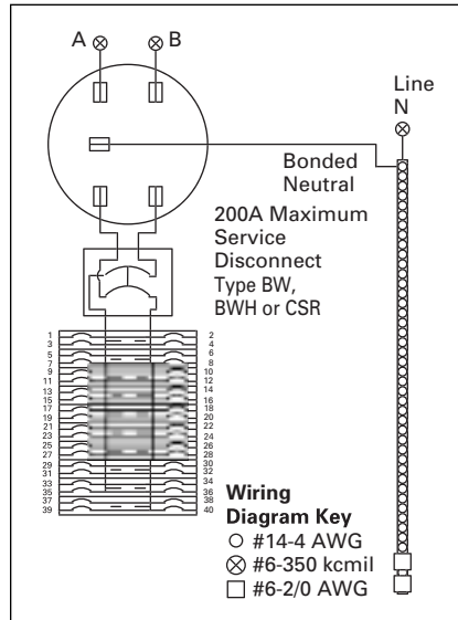
Figure 33. Catalog Numbers – MB2040P200SD, MB2040B200BTS, MB2040P200BTS and MB2040P200BTSD
