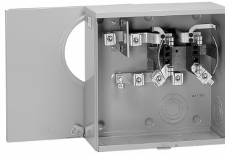
200 Ampere Single-Position Meter Socket (UBHRS223ACH)
