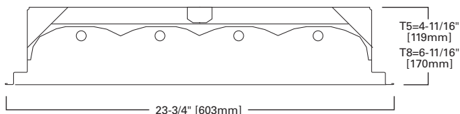
2' x 4', 4 LAMP
