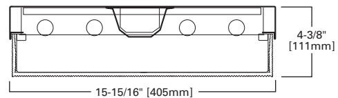
4', 4 LAMP (A)
