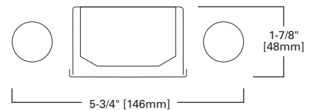
SNSM 2', 3' or 4'
