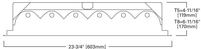
2' x 4', 6 LAMP
