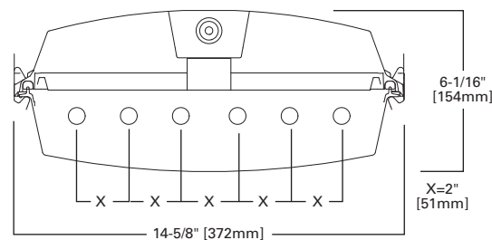
4', 6 LAMP
