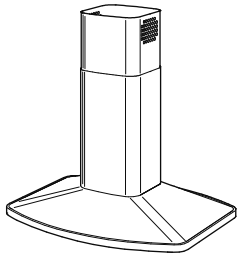
6" Round Duct — Internal Blower High — 480 CFM, 9.5 Sones Low — 230 CFM, 3.0 Sones
