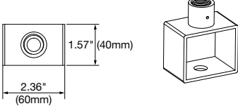
PENDANT MOUNTING BRACKET 100W, 150W, 200W, 240W, 300W
