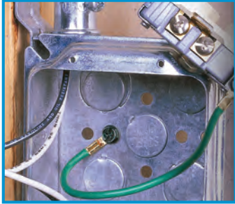
Stranded Wire
