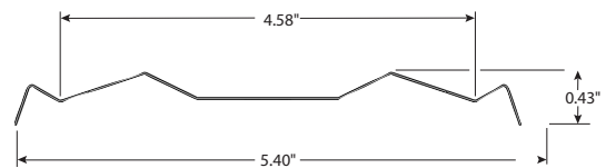
6-inch Reflector
