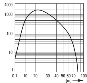
Perfect Prox long range sensor, example
