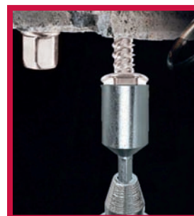
Rod Hanger - Concrete (self-tapping)
