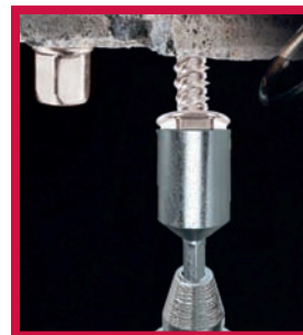
Rod Hanger - Concrete (self-tapping)
